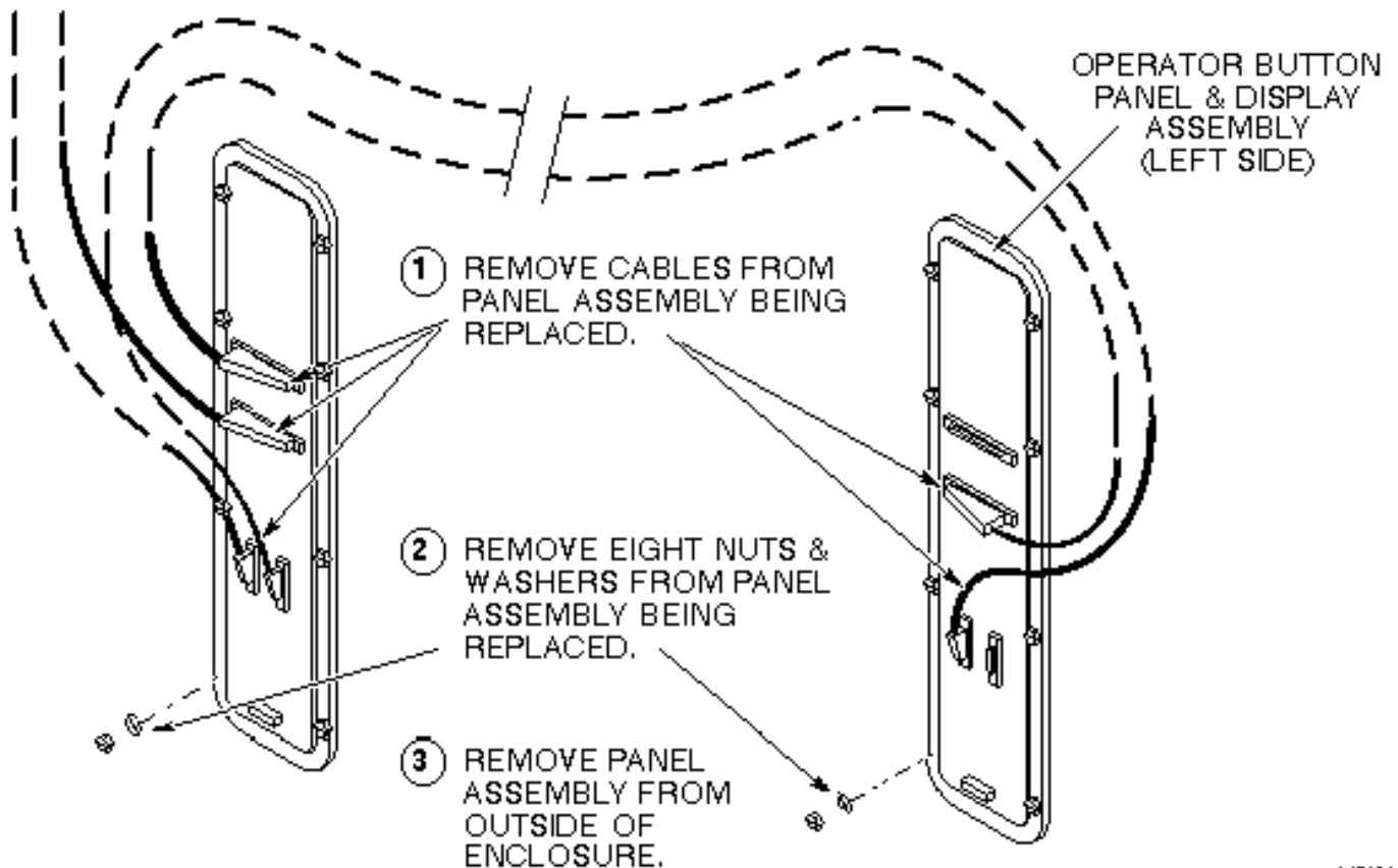
OPERATOR BUTTON PANEL AND DISPLAY ASSEMBLIES ILLUSTRATION L4783A
